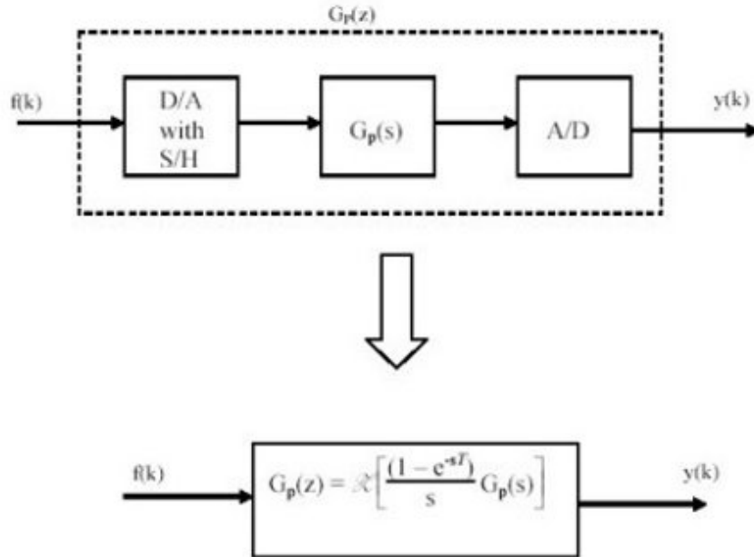
Figure 6: Discretizing a continuous-time plant
