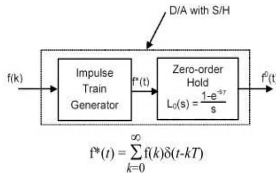
3(b) Representations of a D/A converter with S/H
