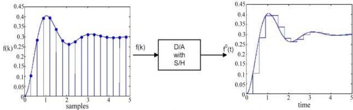
3(a) Symbol for D/A Conversion with S/H
