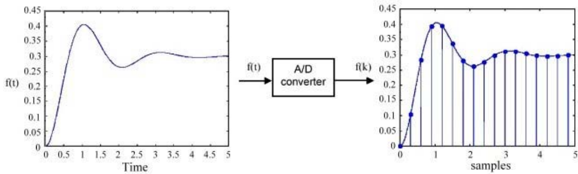
Figure 2: Sampling of a Continuous-Time Signal Using an A/D Converter
